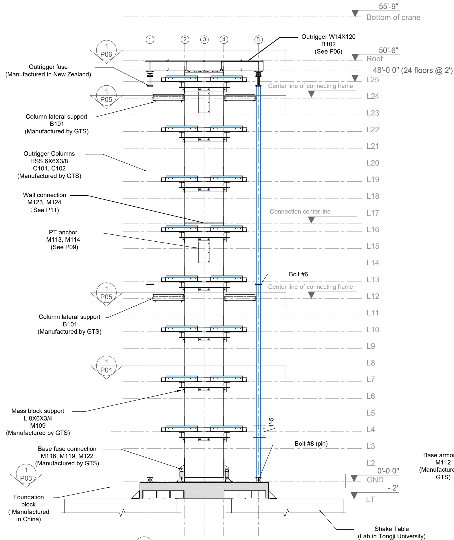
Test set-up: front view
