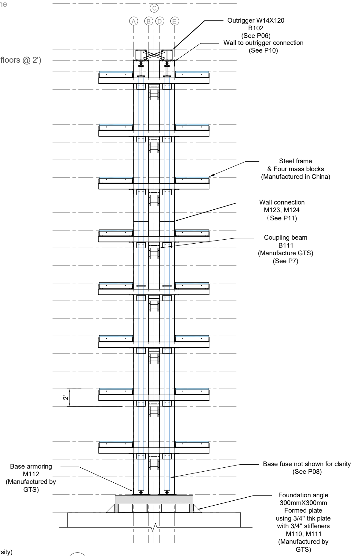
Test set-up: side view
